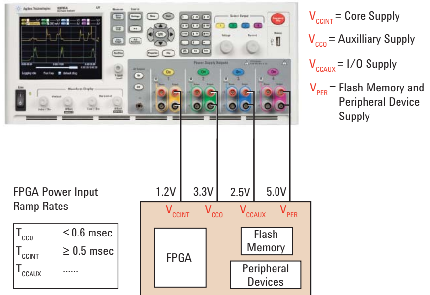
Figure 1. FPGA circuit test setup
