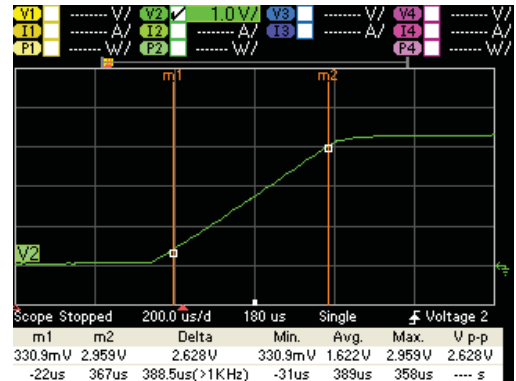
Figure 4. Core voltage and I/O voltage slew rate settings
